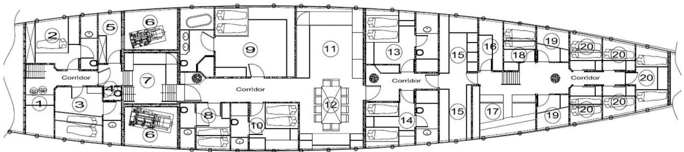
THE 3-MAST SCHOONER " ATLANTIC ", Designed by GARDNER & COX, 1903 Accomodations plan
